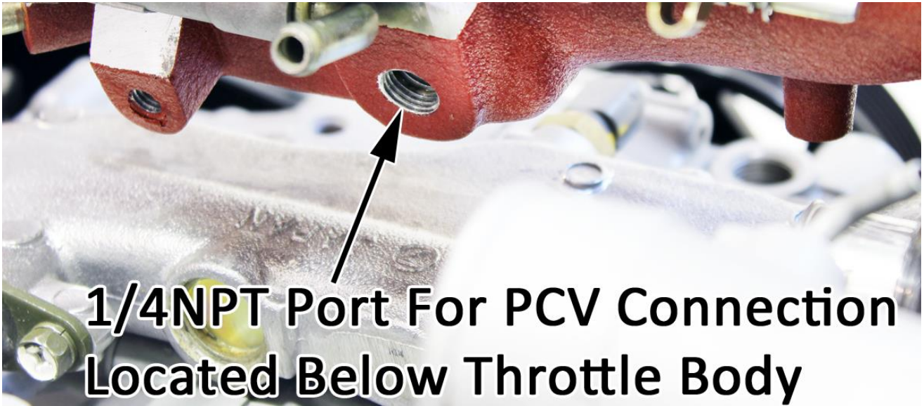
Above picture shows PCV port connection on 2002-07 WRX and STI models.
