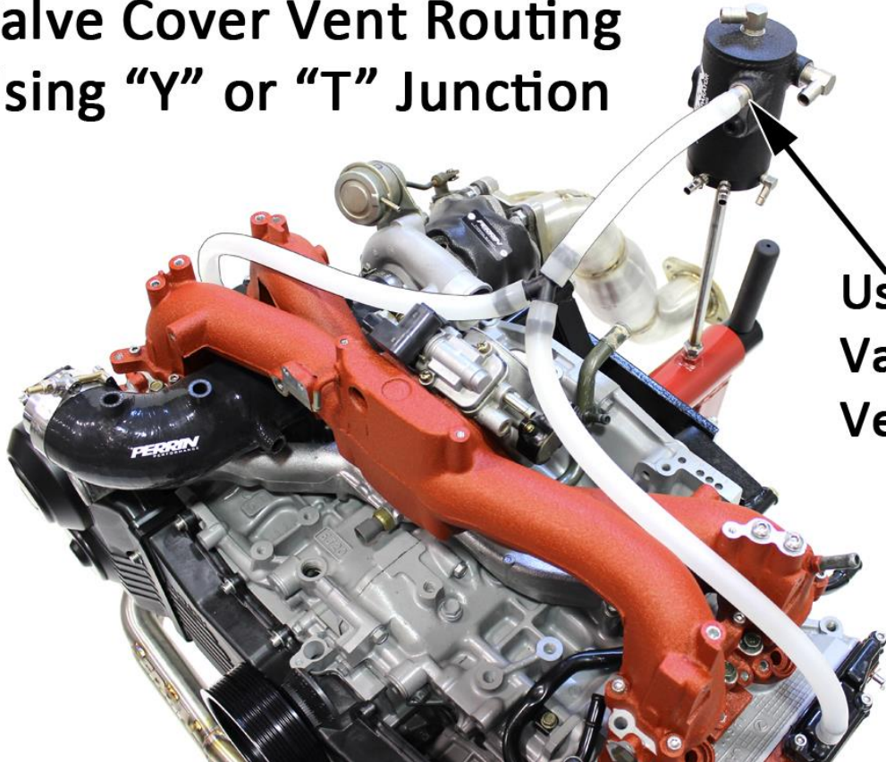
Diagram shows simplified hose routing for 2002-11 WRX and 2004+ STI model.
