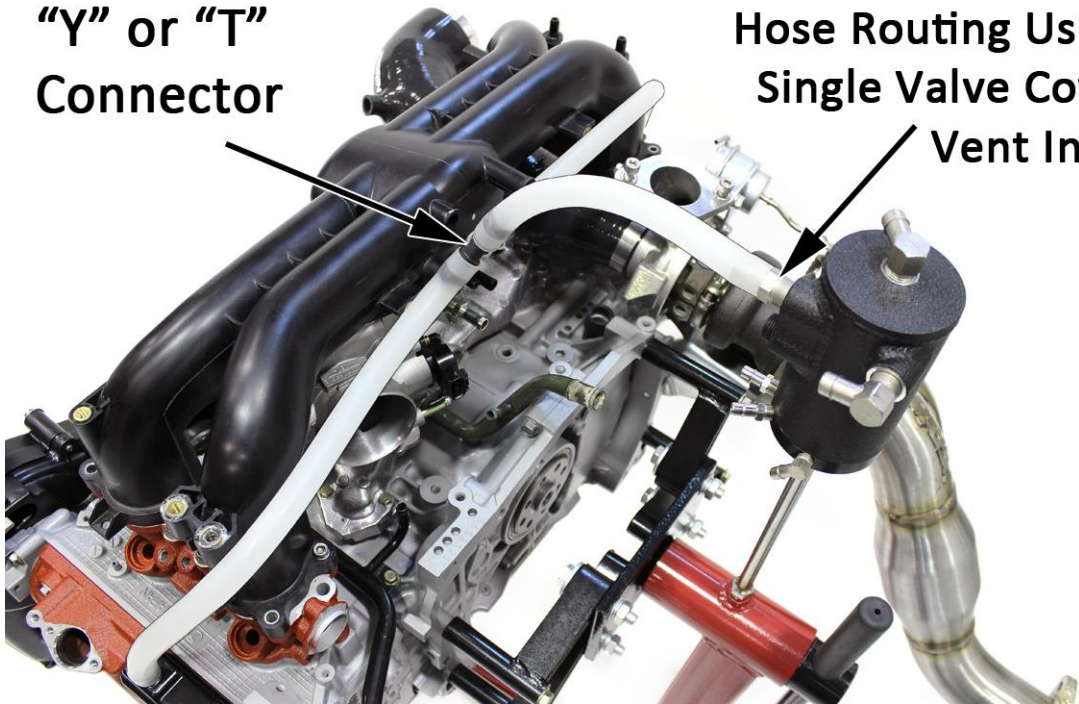
Diagram shows simplified hose routing for 08-14 WRX.
