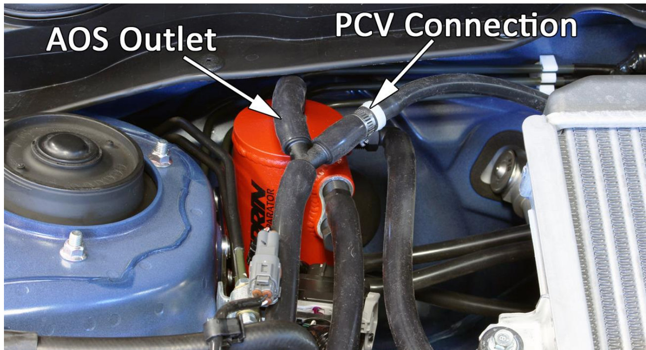
Picture shows another view of the Y junction installed at AOS, and PCV location. PCV location does not need to be this close to AOS.
