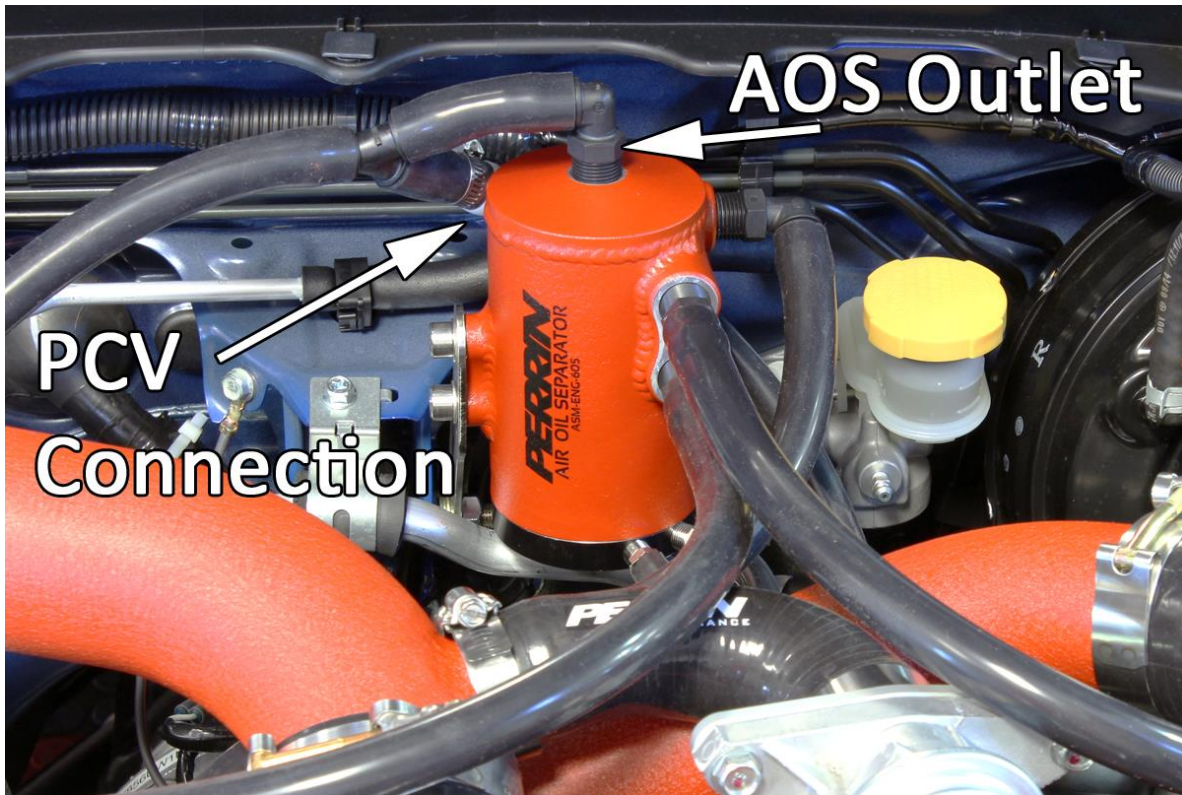
Above picture shows PCV connection on AOS outlet with hose routing behind AOS body.
